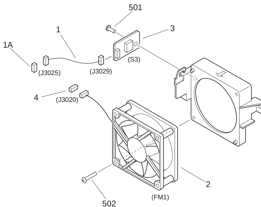
FIGURE 190 DEVELOPING FAN ASSEMBLY
