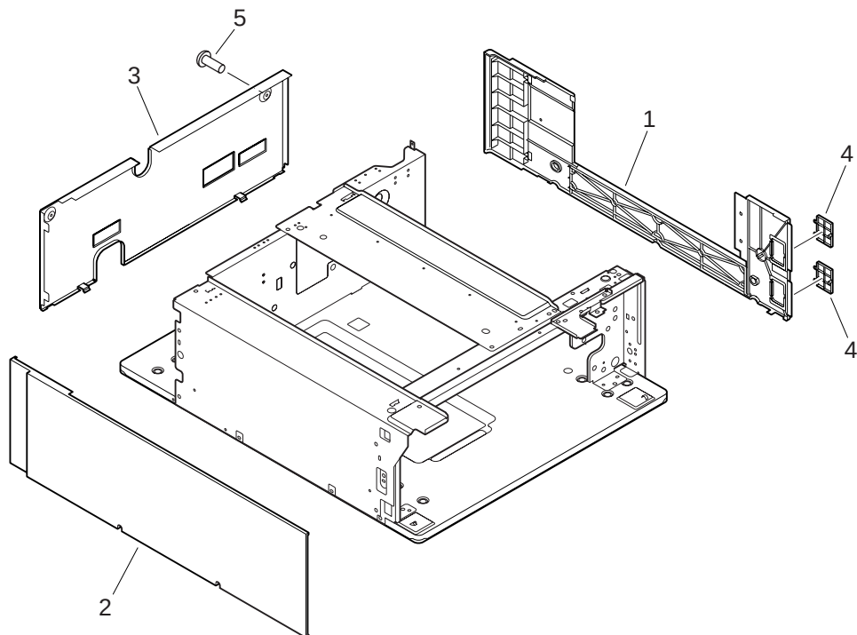
FIGURE Z10 EXTERNAL COVERS, PANELS, ETC.
