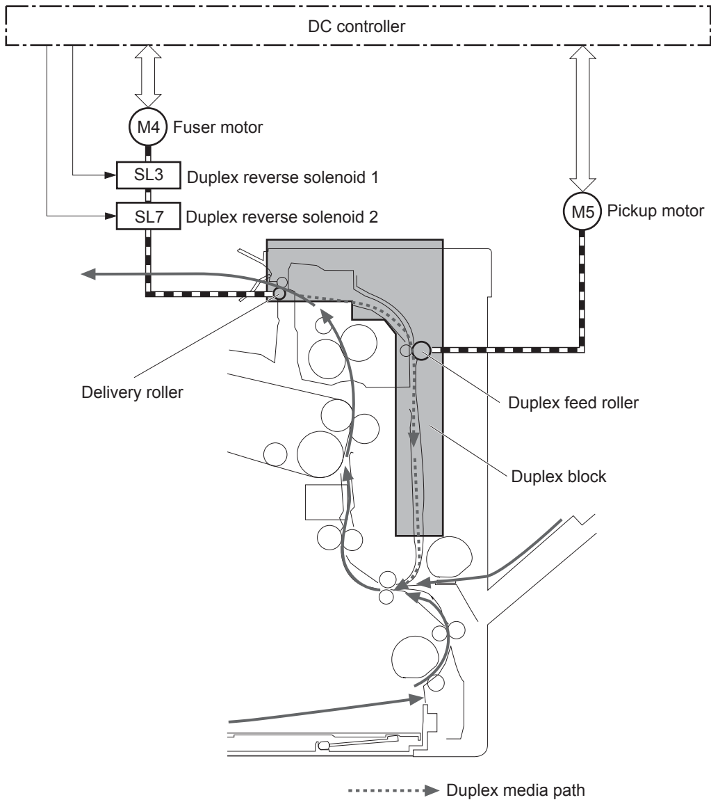
Figure 1-43 Duplex operation
