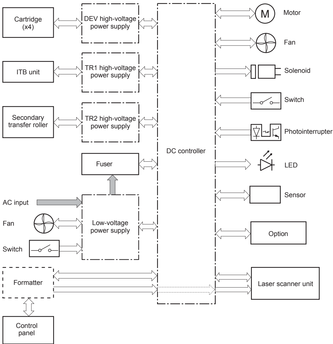
Figure 1-3 DC controller diagram
