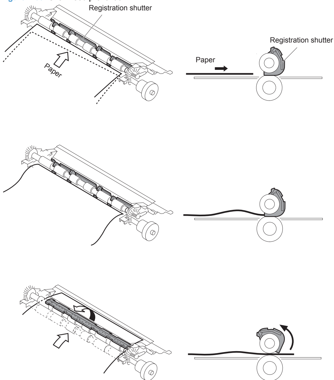
Figure 1-39 Skew-feed prevention
